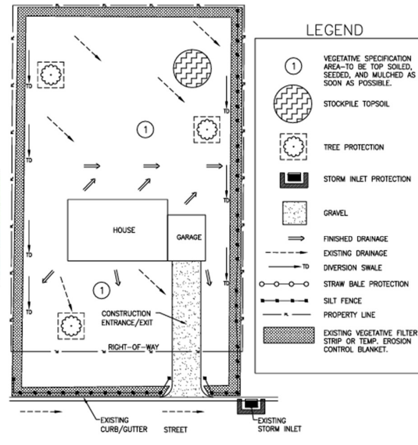
Lot Erosion Control Detail NOT TO SCALE
